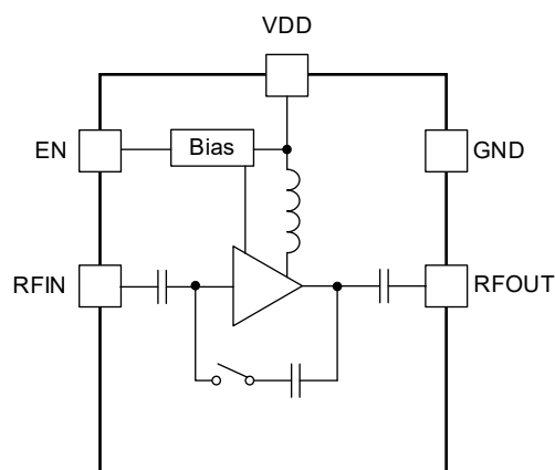
Figure 1. SGM13005H2 Block Diagram
