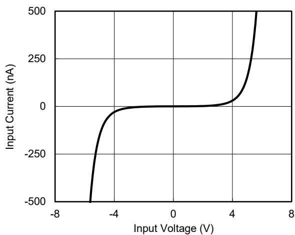
IV Curve
