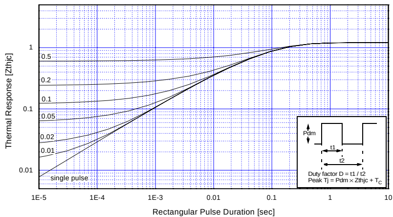
Fig 17. Transient Thermal Impedance of IGBT
