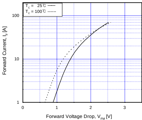
Fig 18. Forward Characteristics
