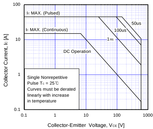
Fig 15. SOA Characteristics
