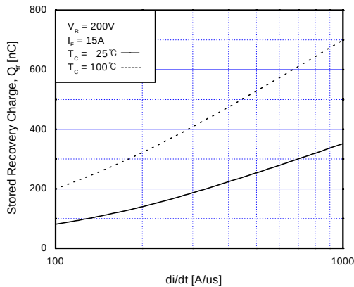
Fig 20. Stored Charge
