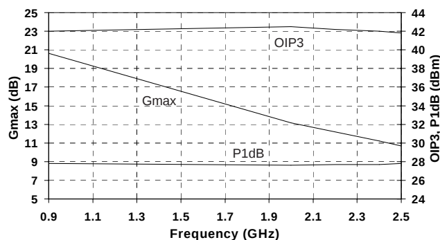
Typical Gmax, OIP3, P1dB @ 5V, 270mA
