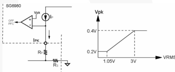
FIG.6 Current Limit
