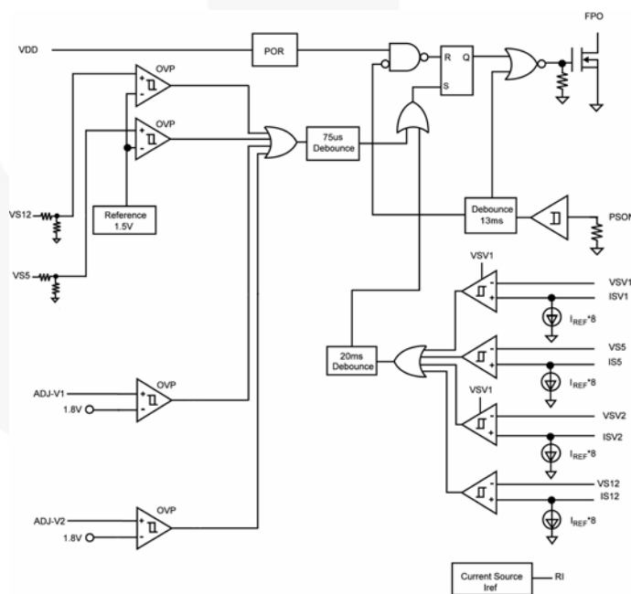
Figure 2. Function Block Diagram
