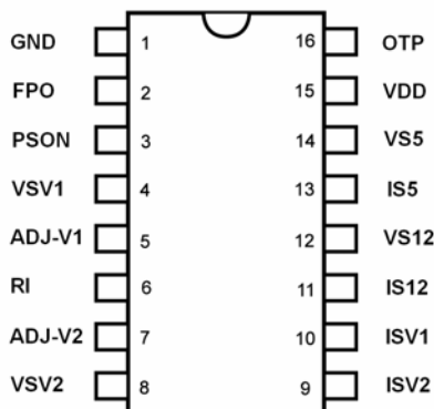
Figure 3. Pin Configuration
