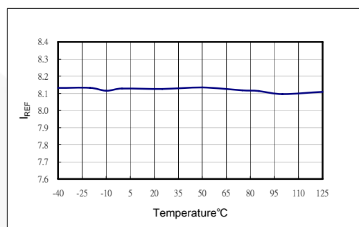
Figure 6. Ratio of Sense Sink Current Sense Setting Pin (RI) Source Current
