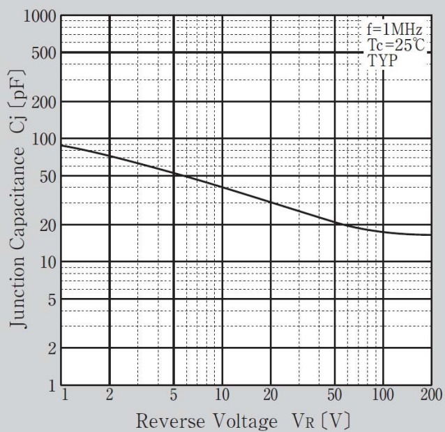
Junction Capacitance
