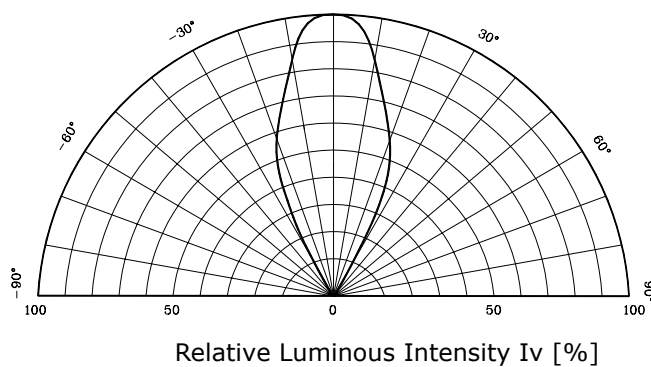
Fig. 5-1 Radiation Diagram
