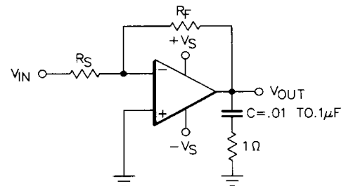
FIGURE 8 - INVERTING AMPLIFIER WITH RC LOAD COMPENSATION
