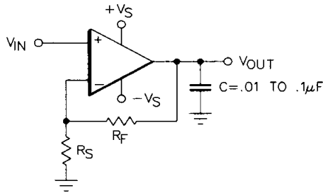
FIGURE 9 - NON-INVERTING AMPLIFIER WITH CAPACITIVE LOAD COMPENSATION
