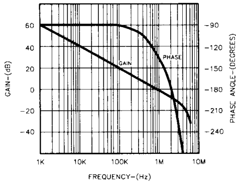
FIGURE 1. FREQUENCY RESPONSE
