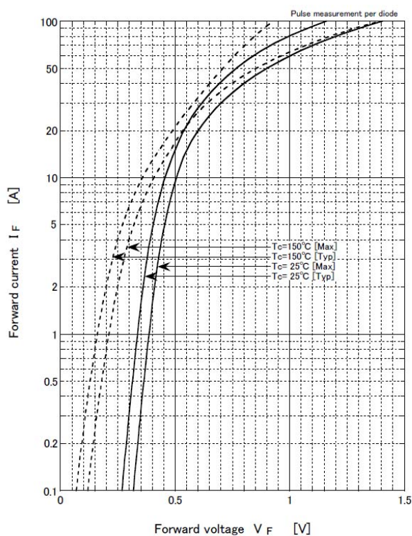
Forward voltage
