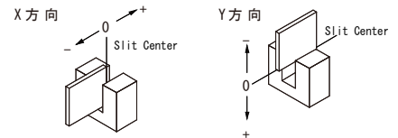
*2 Method of Measuring Position Detection Characteristic
