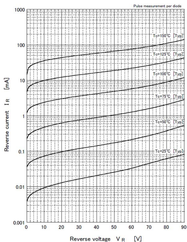
Reverse current
