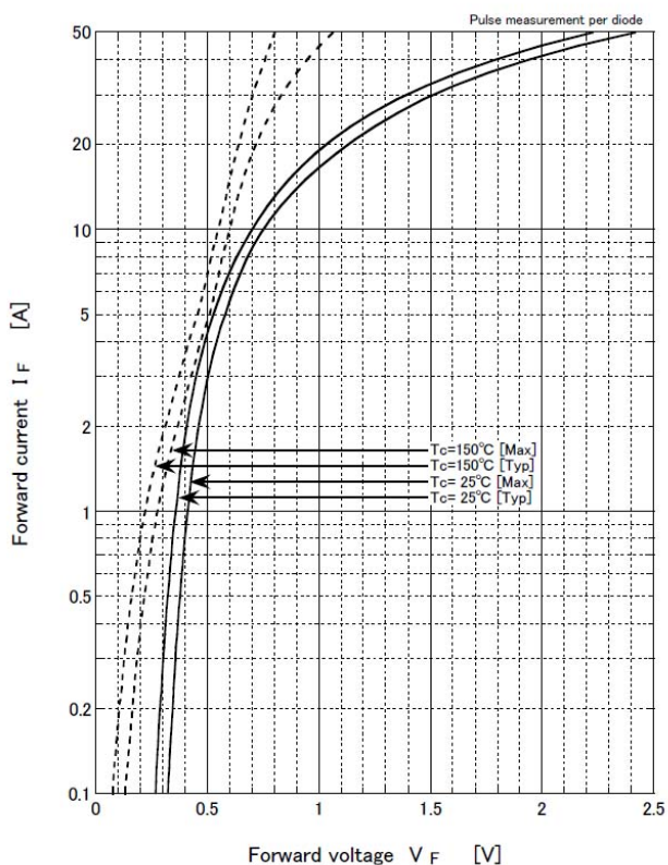
Forward voltage
