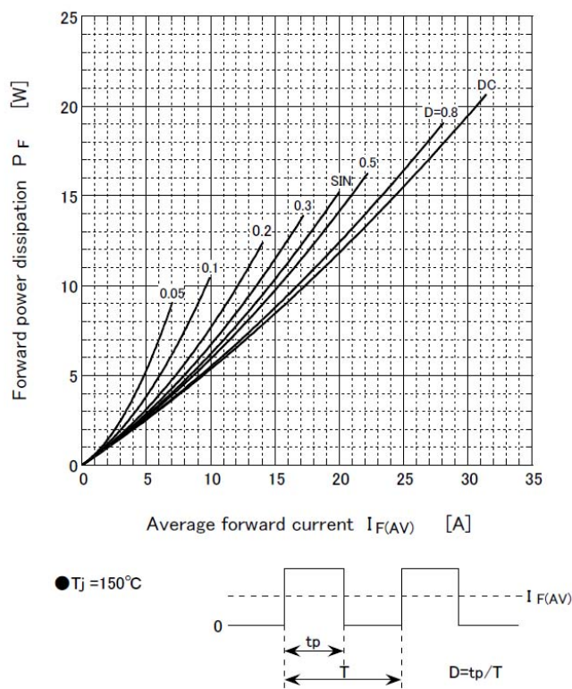
Forward power dissipation
