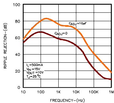
Figure 8 – Ripple Rejection vs. Frequency
