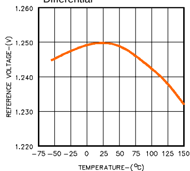
Figure 5 – Reference Voltage vs. Temperature
