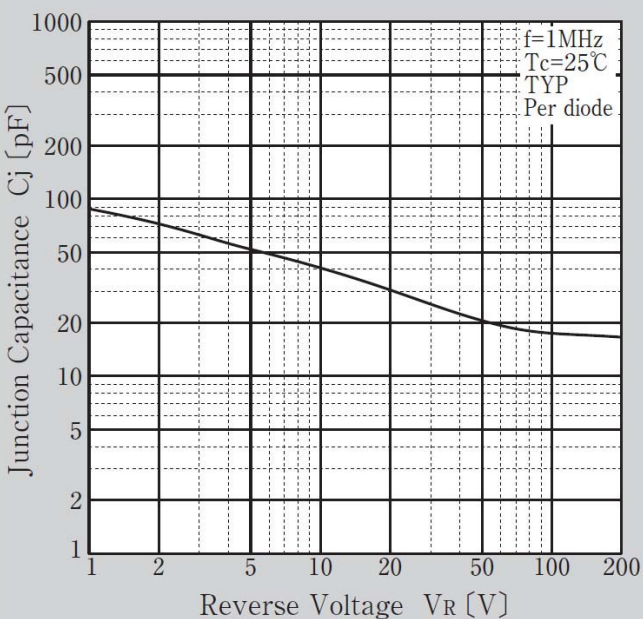
Junction Capacitance
