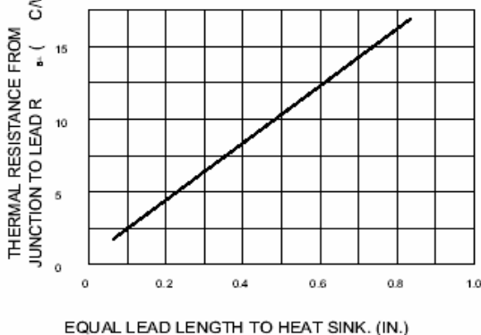
FIG.5-TYPICAL THERMAL RESISTANCE
