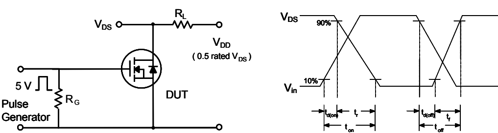
Fig 13. Switching Time Test Circuit & Waveforms
