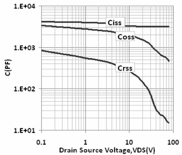
Figure 2. Capacitance Characteristics
