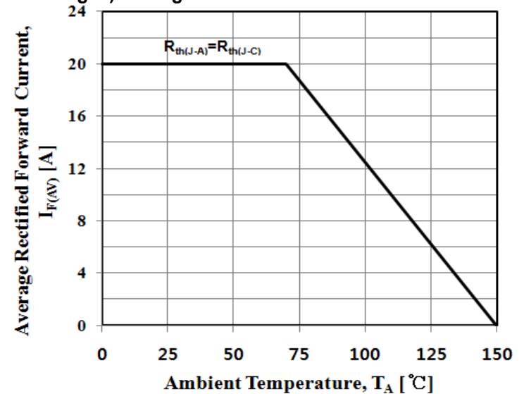
Fig. 6) Average Forward Current Characteristics
