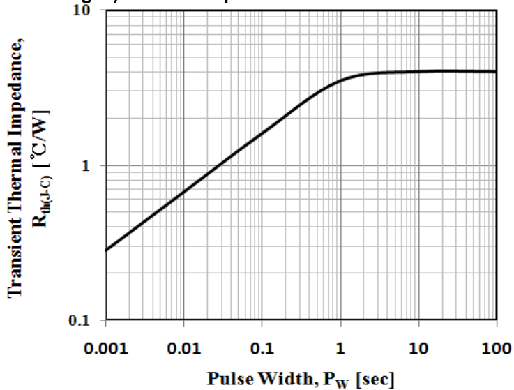
Fig. 5) Thermal Impedance Characteristics
