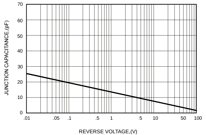
FIG.5-TYPICAL JUNCTION CAPACITANCE
