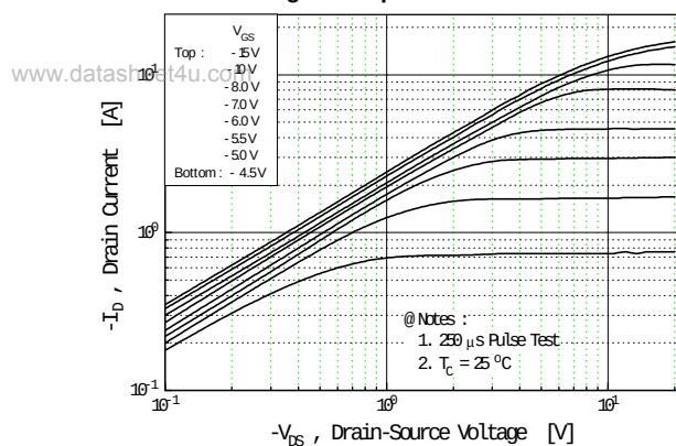
Fig 1. Output Characteristics
