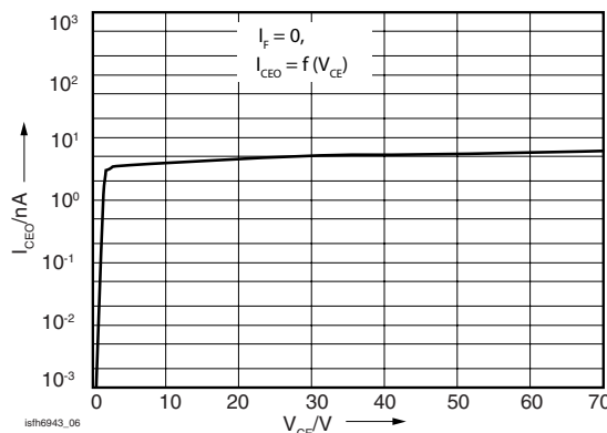
Figure 6. Collector-Emitter Leakage Current (typ.)
