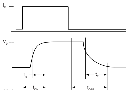
Figure 2. Switching Waveform
