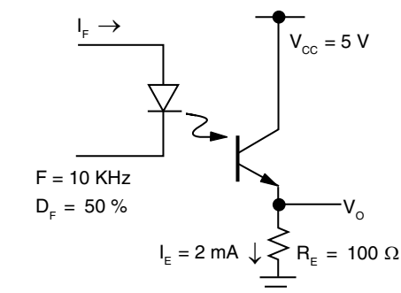
Figure 1. Switching times (typ.)
