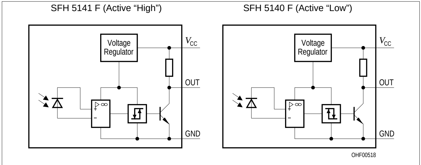
Figure 1 Block Diagram
