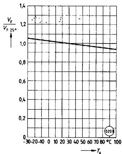
Forward voltage versus ambient temperature
