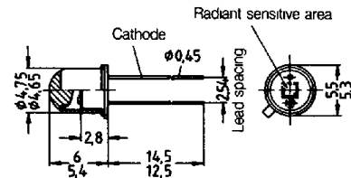
Package Dimensions mm
