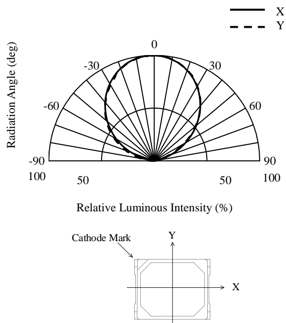
Figure 13. Directivity ( T_A = 25\text{ }^{\circ}\text{C} , I_F = 30\text{ mA} )
