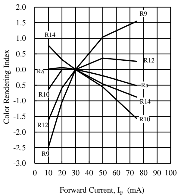
Figure 10. Color Rendering Index vs. I_F
