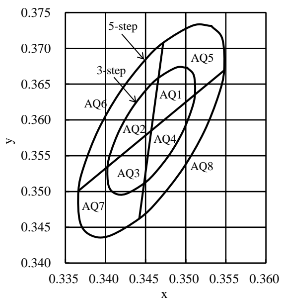
Figure 2. Chromaticity Diagram
