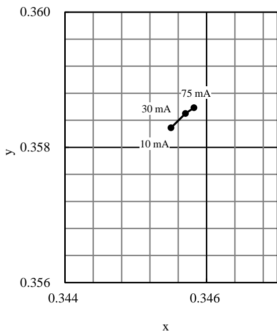
Figure 8. I_F vs. Chromaticity ( T_A = 25\text{ }^{\circ}\text{C} )
