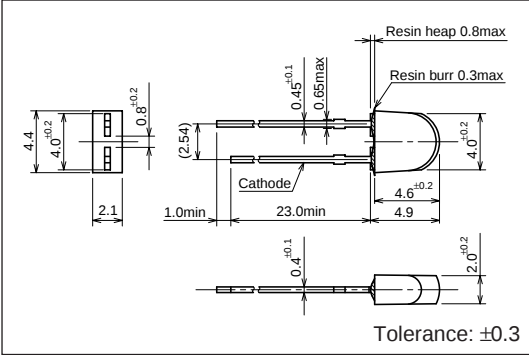
External Dimensions (Unit: mm)
