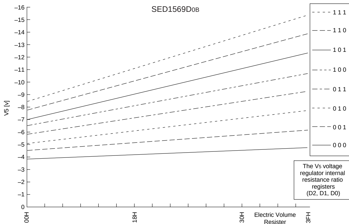
Figure 19: SED1569D0B (Temperature Gradient = -0.05\%/^{\circ}\text{C} Model)
