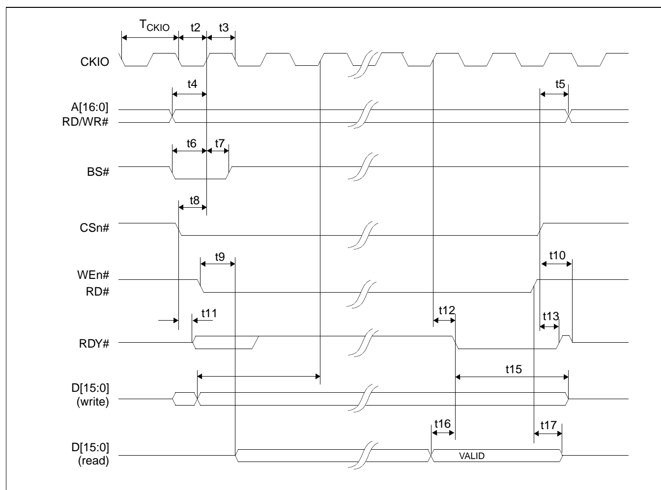
Figure 7-1: SH-4 Timing
