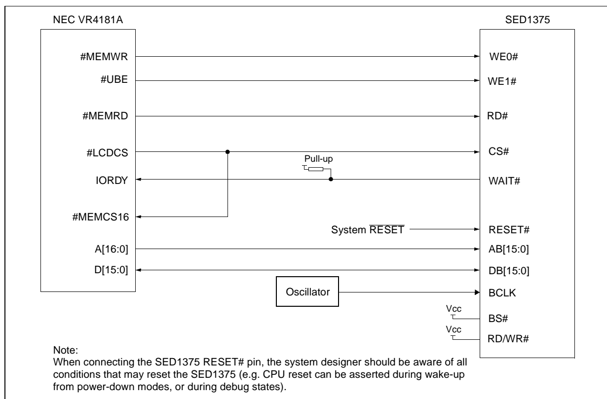
Figure 4-1: Typical Implementation of VR4181A to SED1375 Interface
