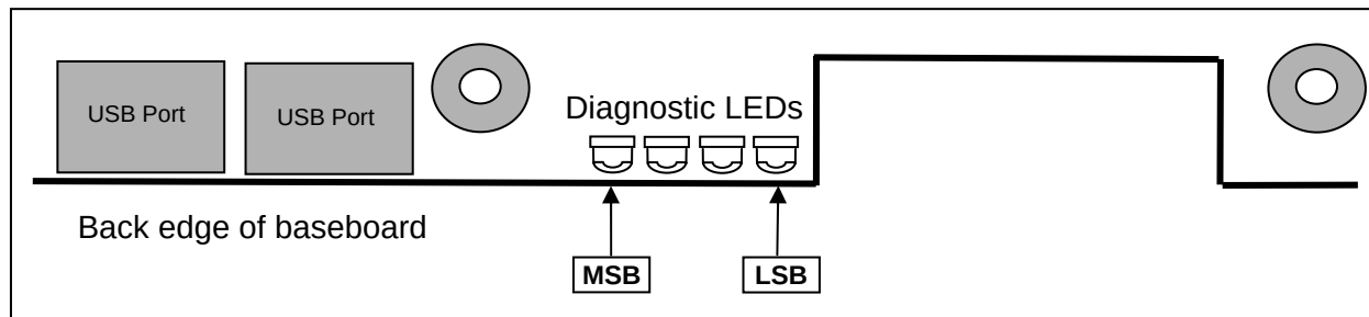
Figure 6. Location of Diagnostic LEDs on Server Board
