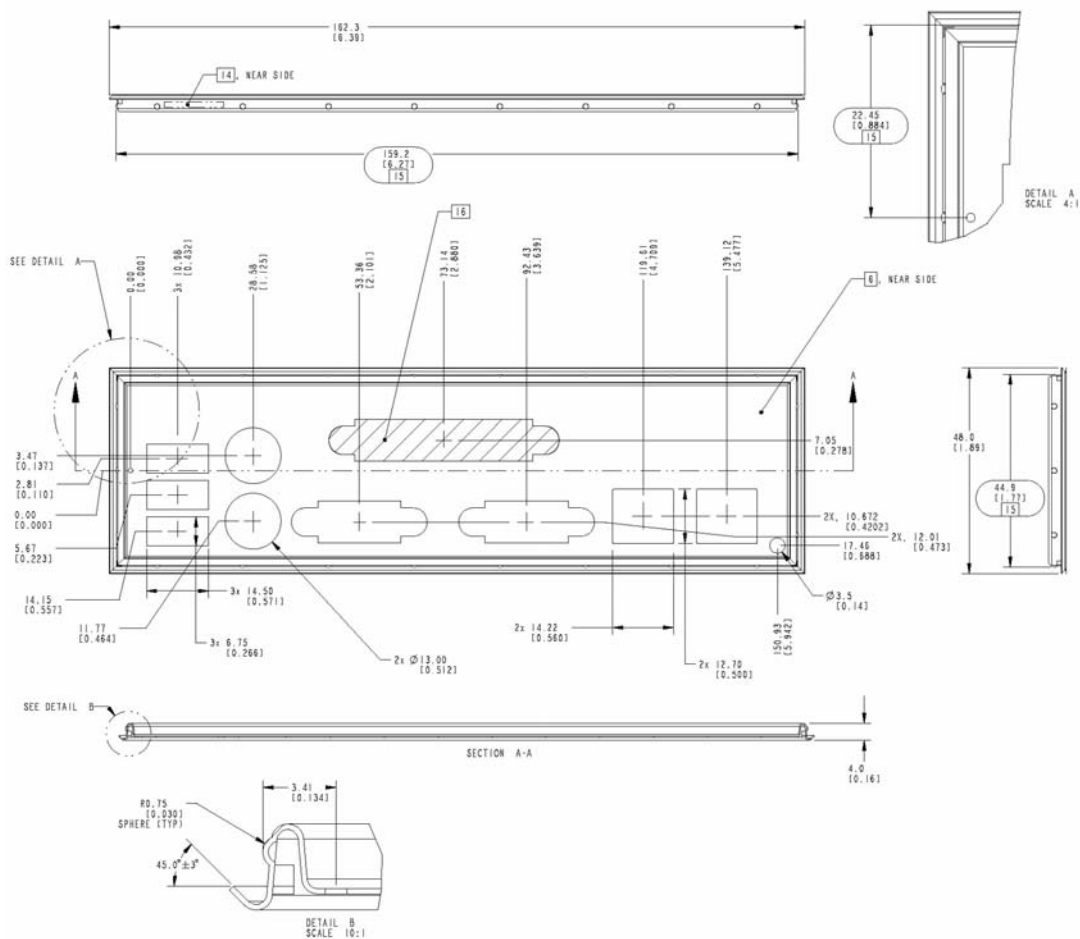
Figure 14. Intel Server Board SE7210TP1-E I/O Shield Drawing
