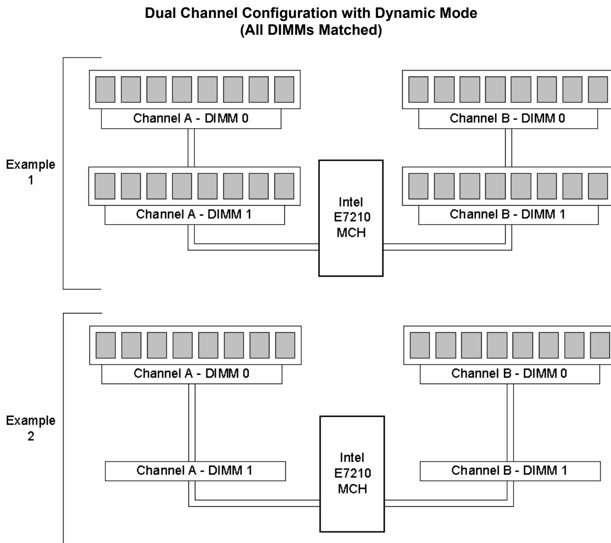
Figure 5. Examples of Dual Channel Configuration with Dynamic Mode
