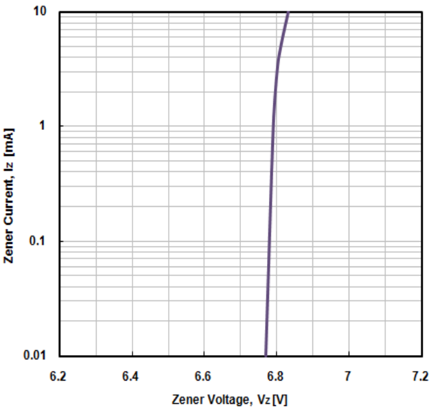
Fig. 1) Typical Zener Characteristics
