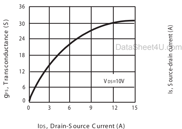
Figure 7. Transconductance Variation with Drain Current
