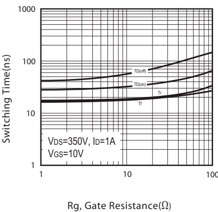
Figure 11. switching characteristics
