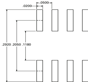
5x6 QFN Solder Pad Layout
