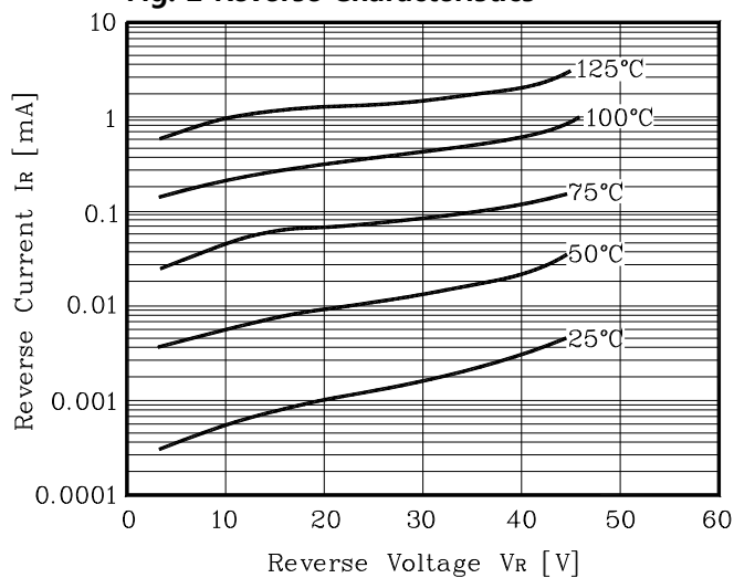
Fig. 2 Reverse Characteristics
