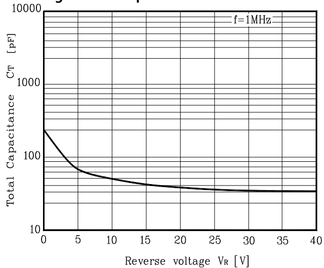
Fig. 3 Total Capacitance
