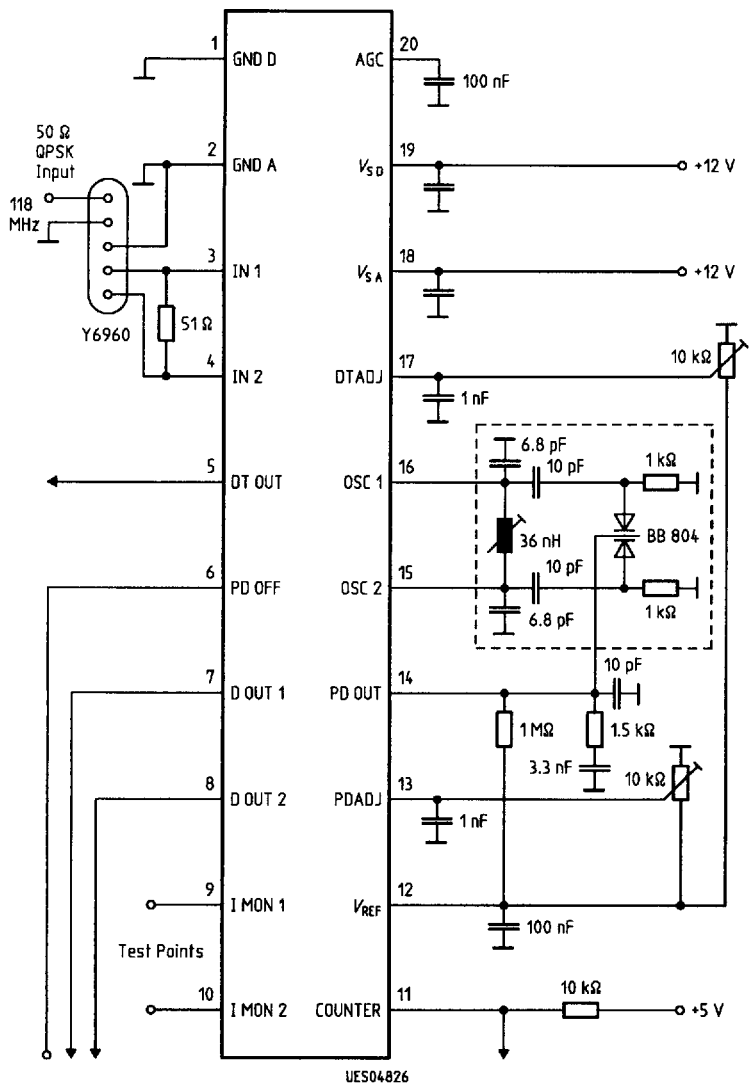
Application Circuit 118 MHz
