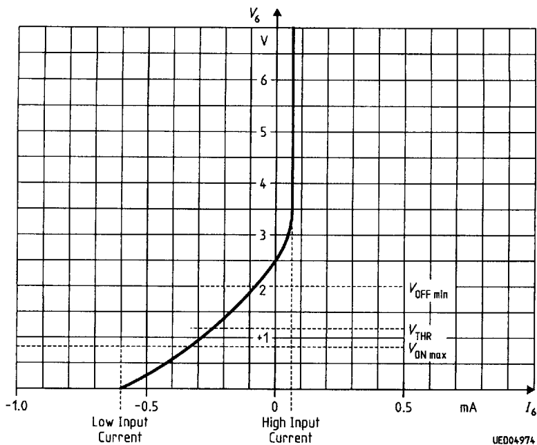
Note 4 PD OFF Input Characteristic
