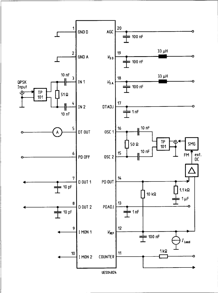
Test Circuit
