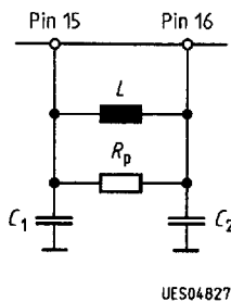
Note 5 Application Circuit for use of Internal Oscillator (not subject to production testing)
