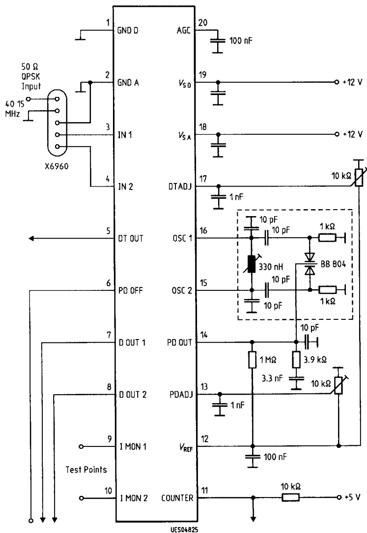
Application Circuit 40.15 MHz
