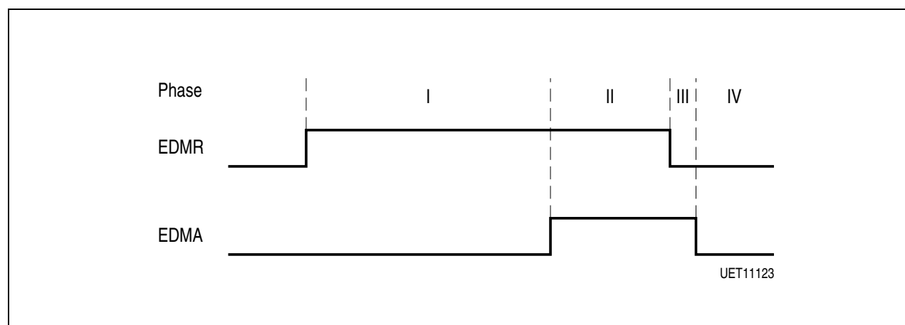
Figure 4-9 Four-Phase Handshake
