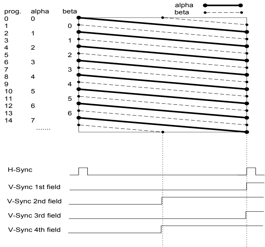
Figure 9-3 50Hz/100Hz mode(ABAB)
