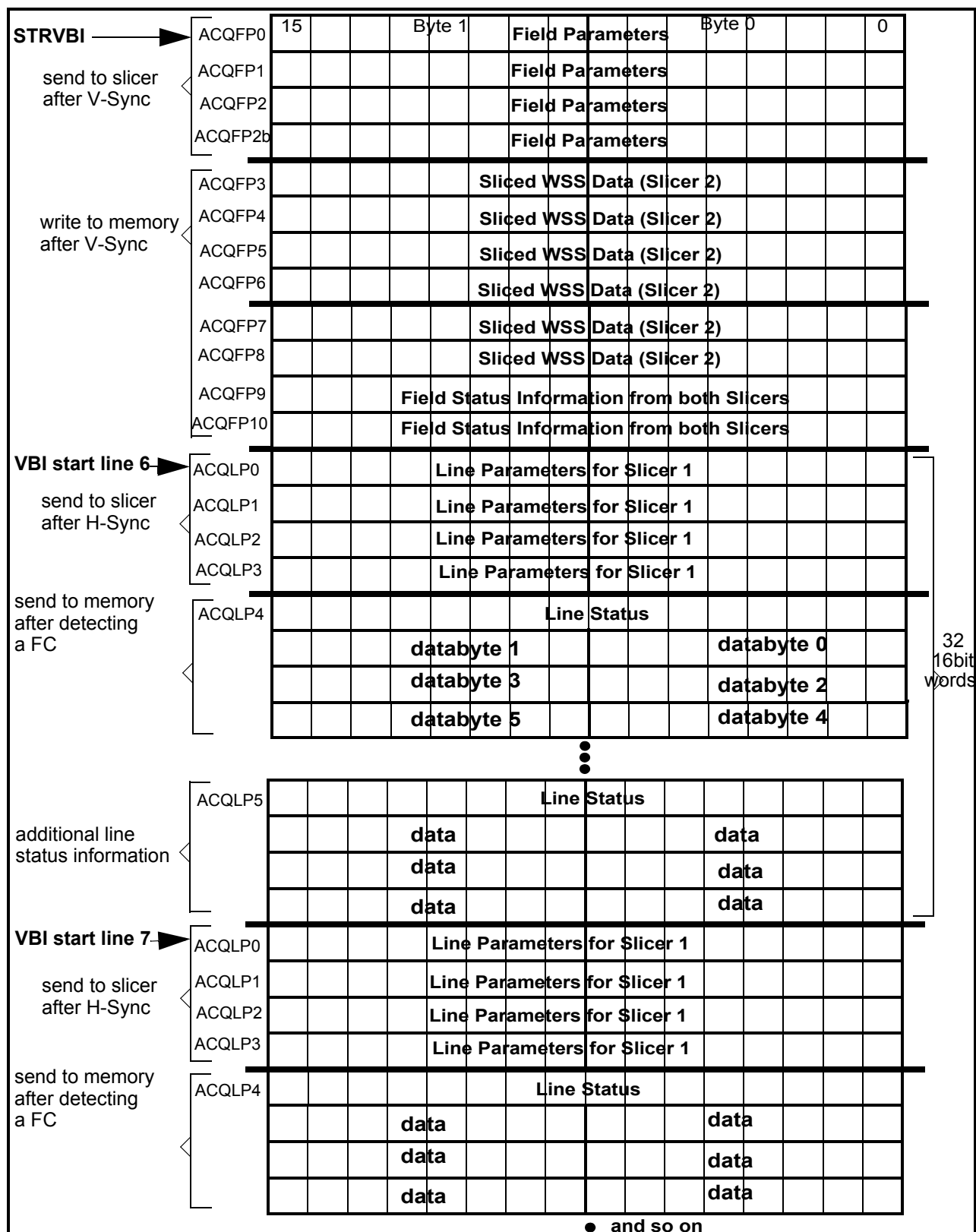
Figure 12-2 VBI Buffer: General Structure
