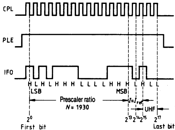
Pulse diagram
