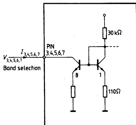
Test circuit 3
