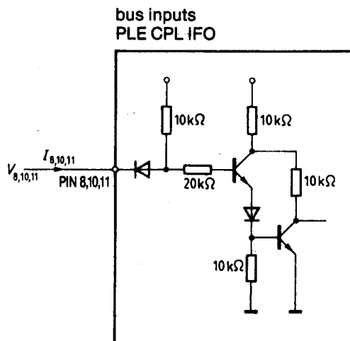
Test circuit 2
