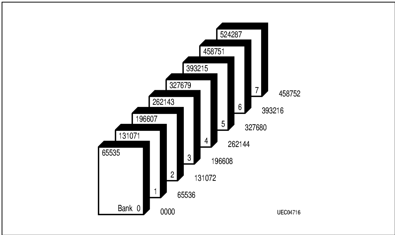
Figure 5 Bank Organization
