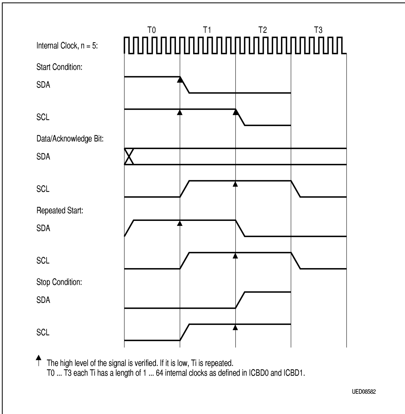
Figure 29 I²C Bus Events
