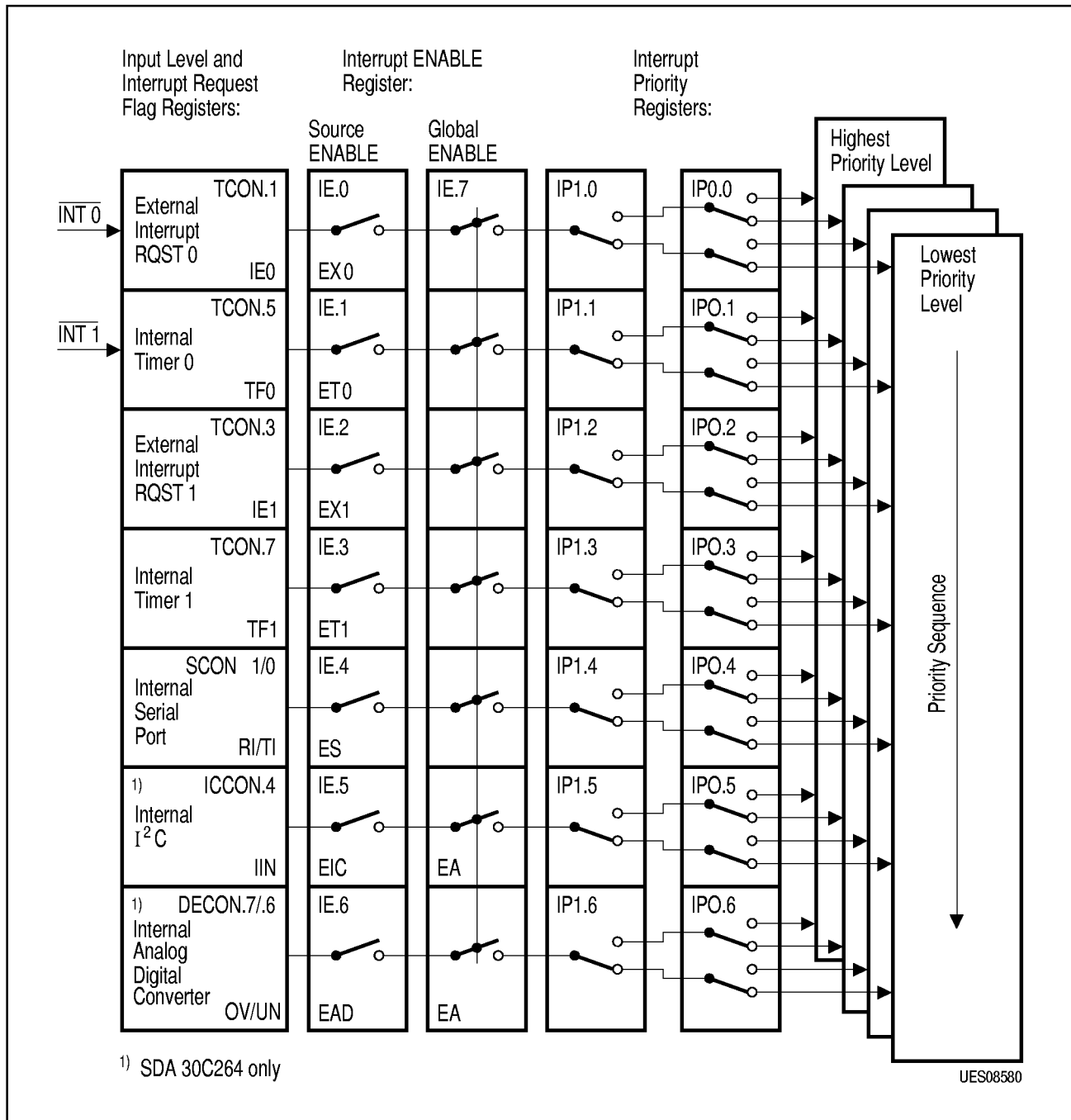
Figure 13 Interrupt System
