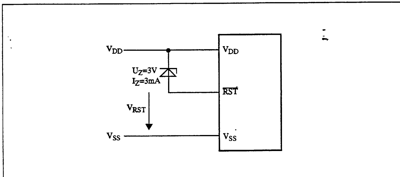
Figure 15 Power-On Reset Circuit
