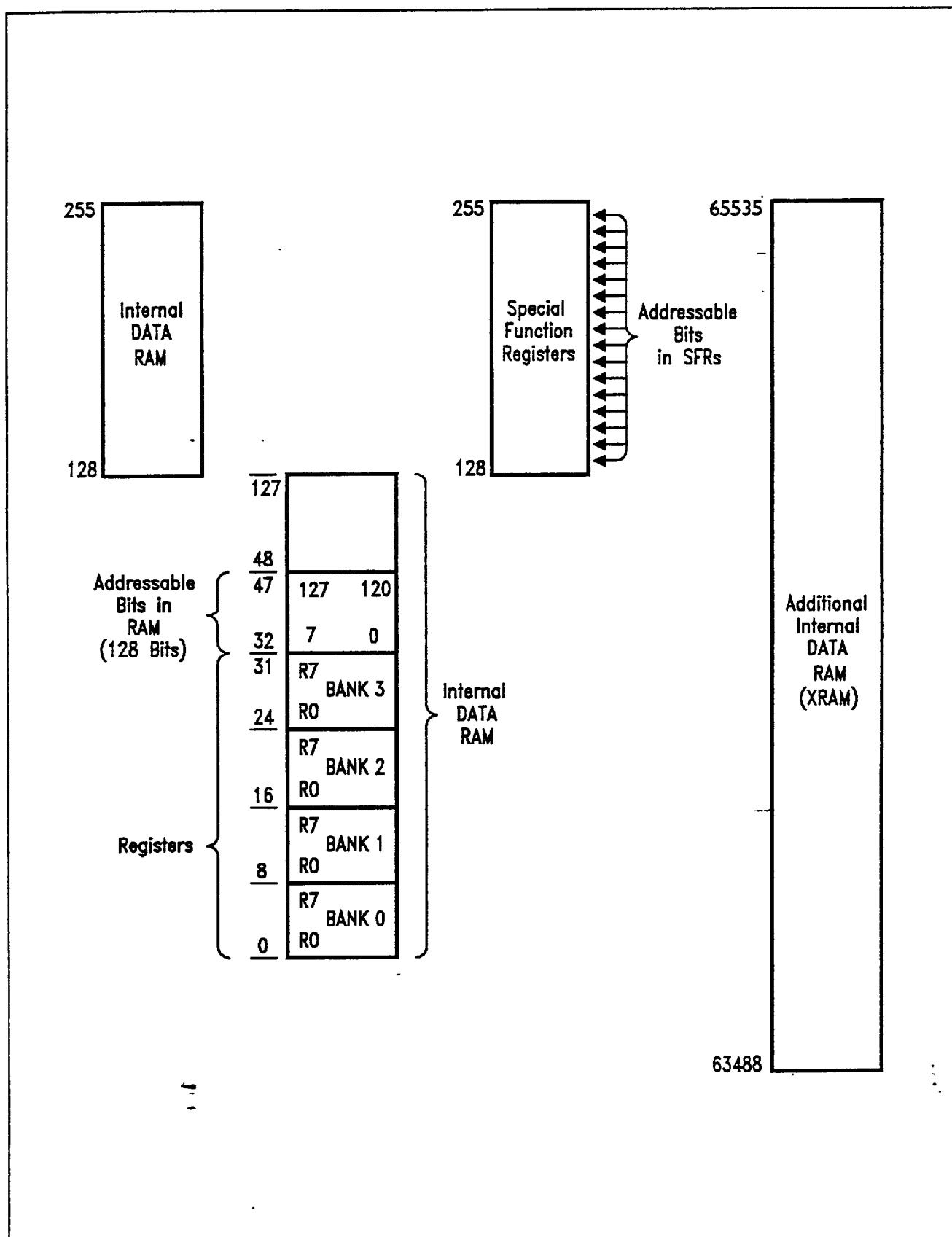
Figure 8 Internal Data Memory Address Space
