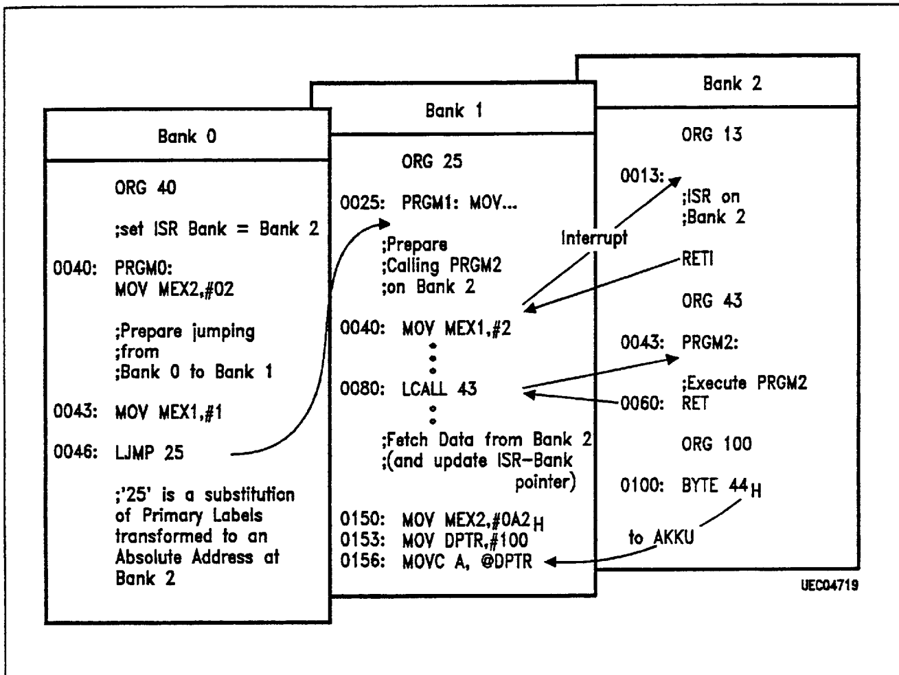
Figure 7 Program Example
