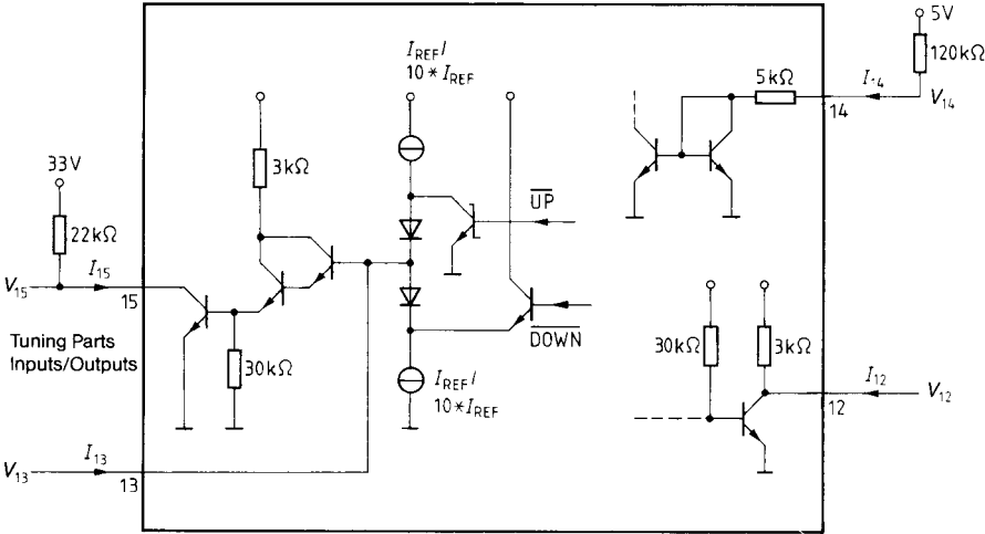
Test circuit 5
