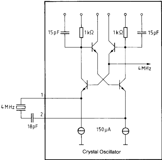
Test circuit 4
