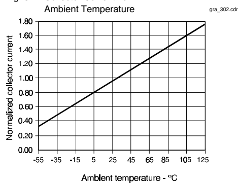
Fig. 8 Collector Current vs Ambient Temperature
