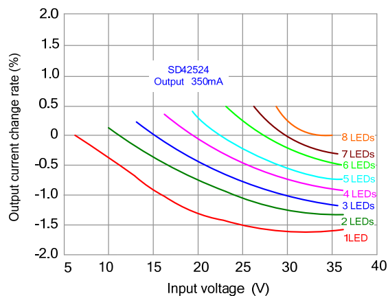
Output 350mA current change rate following the input voltage change
