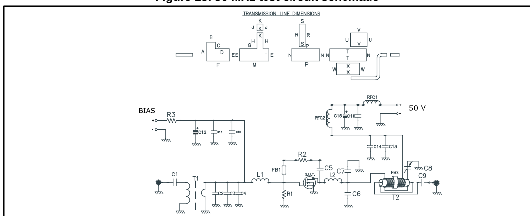
Figure 13: 30 MHz test circuit schematic
