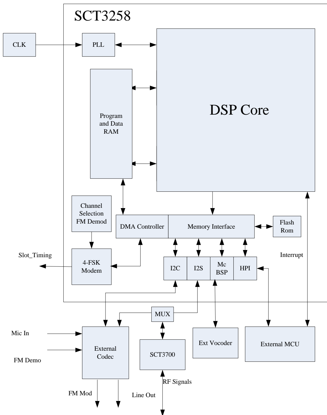
Figure 3-1 SCT3258 Architecture
