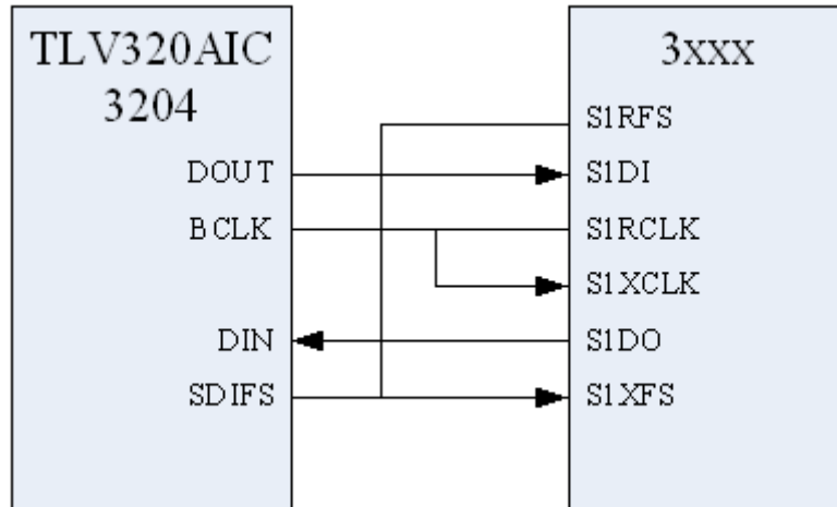
Figure 9-2 TLV320ACI3204 Connection Diagram
