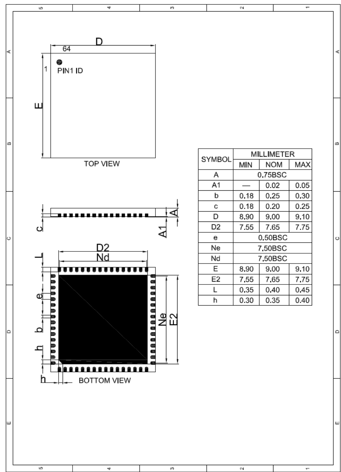
Dimensions shown in millimeters Figure 15-1 SCT3258 QFN64 Package
