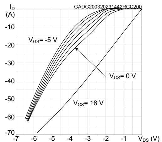
Figure 18. Typical reverse conduction characteristics (Tj = 200 °C)
