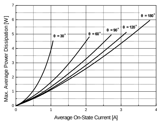
Fig 8. Power Dissipation
