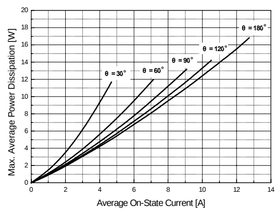
Fig 8. Power Dissipation
