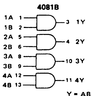
FUNCTION DIAGRAMS
