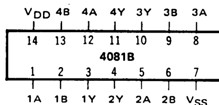
CONNECTION DIAGRAMS
