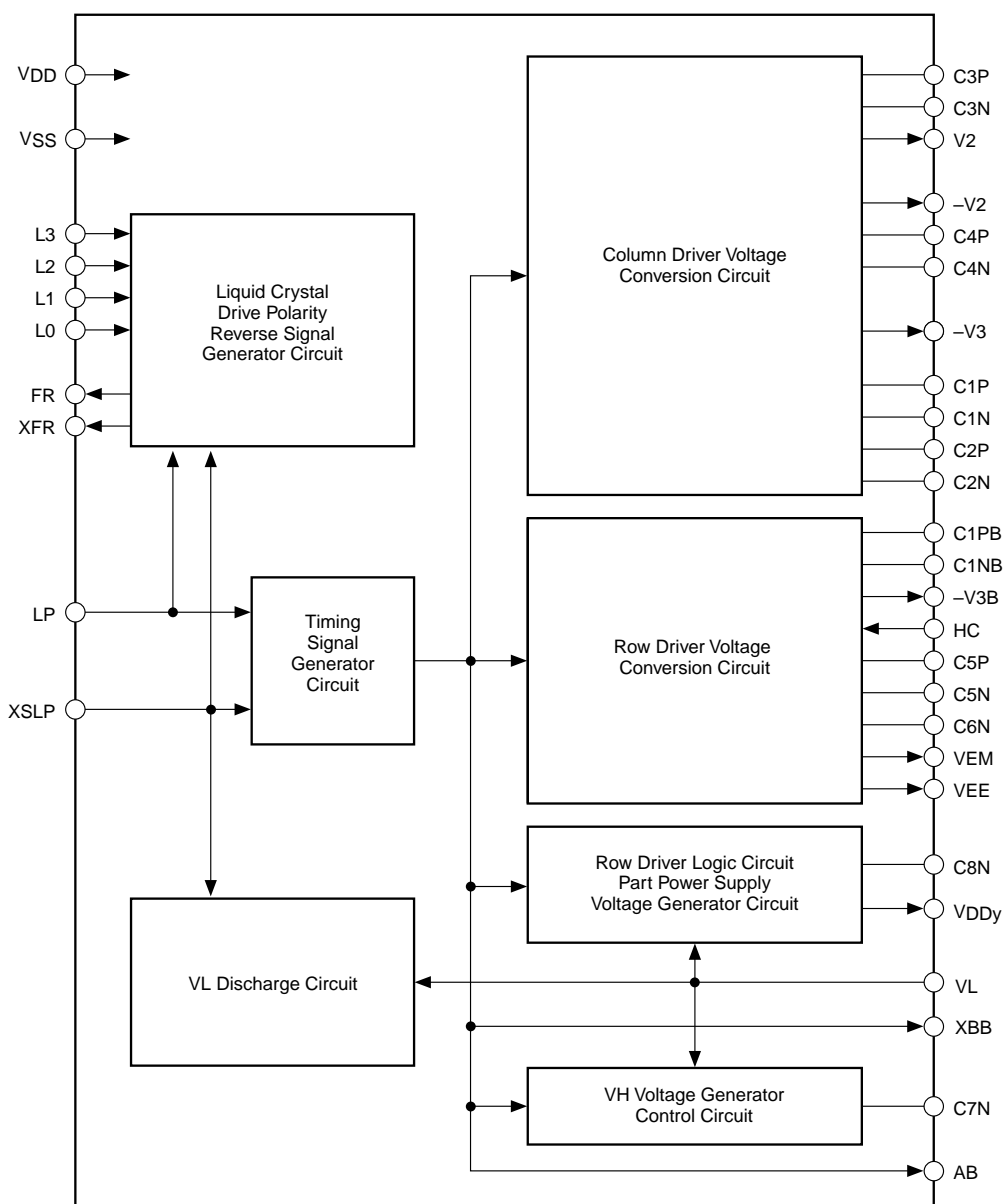
Figure 1: Block Diagram
